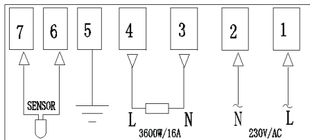
Electric Heating System
