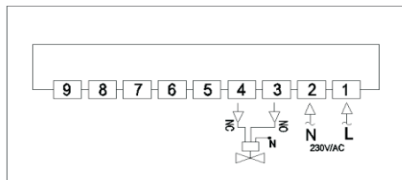
Water Heating System
